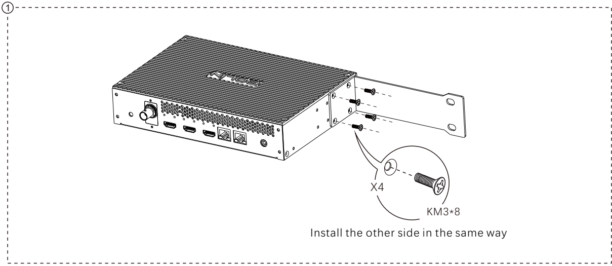
Single Device Mounting Bracket x 2
