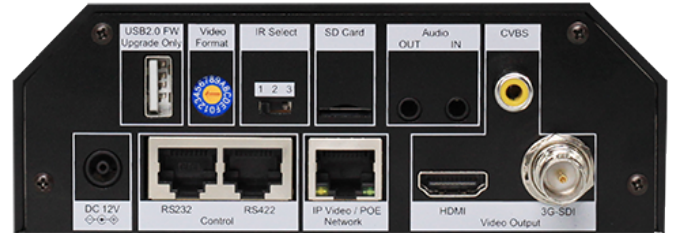
Back Panel
